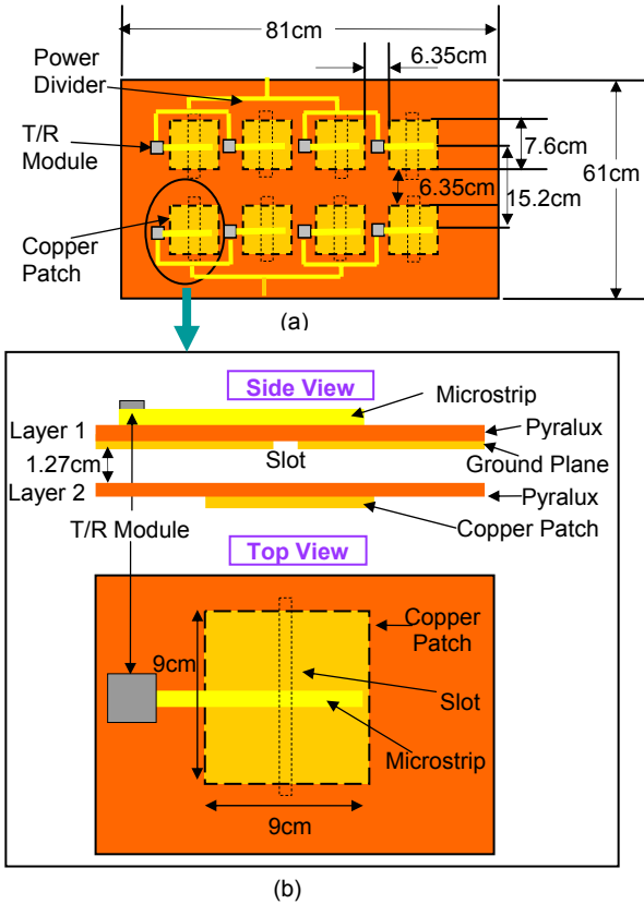
Fig. 2. Membrane antenna architecture. (a) 2x4 element array. (b) Unit cell top and side views.
