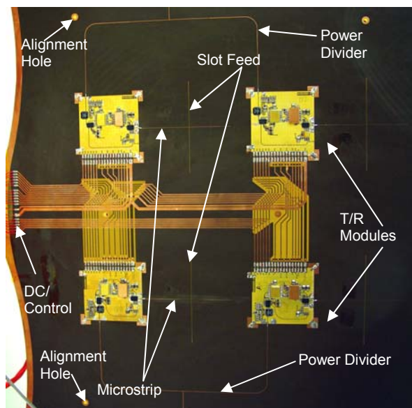
Fig. 6. A close-up of the membrane array showing four of the T/R modules of the array.
