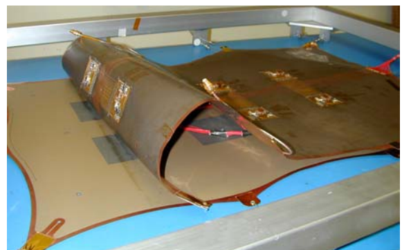
Fig. 5. Antenna in rolled configuration
