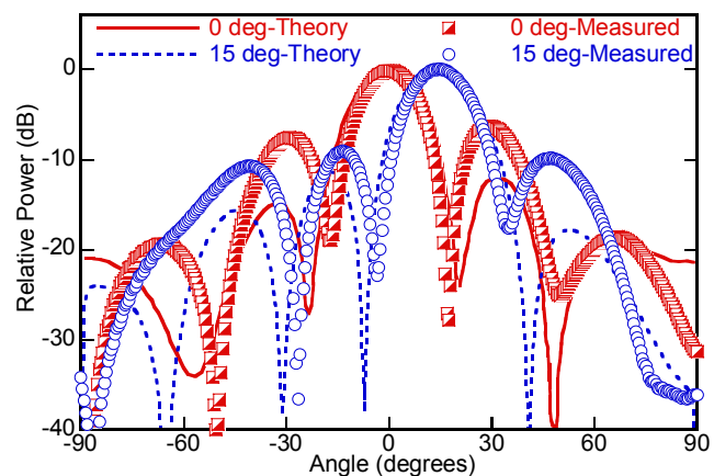
Fig. 8. Measured and theoretical transmit antenna patterns for 0^\circ and 15^\circ steering angles.
