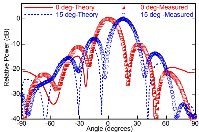
Fig. 7. Measured and theoretical receive antenna patterns for 0^\circ and 15^\circ steering angles.
