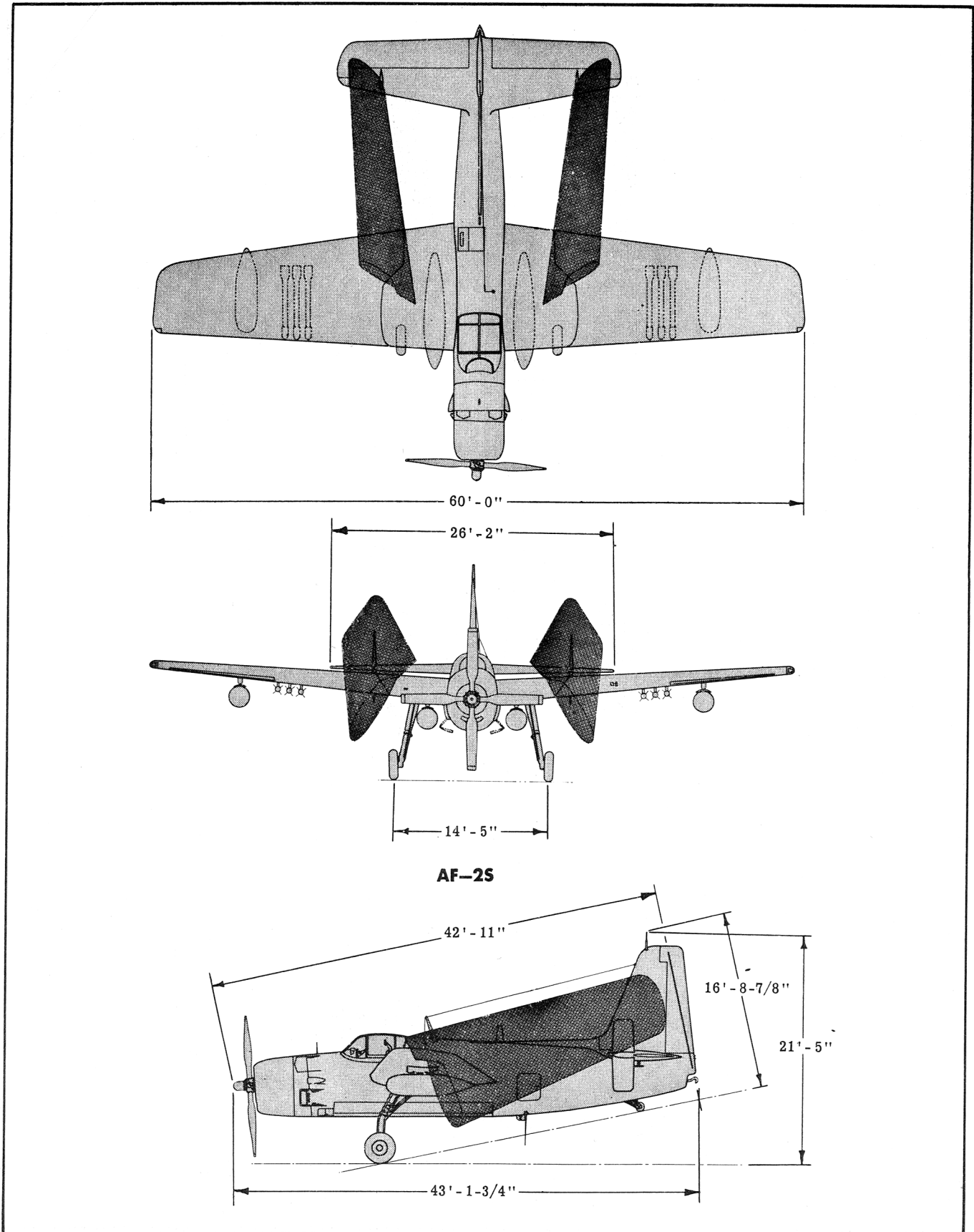
Figure 1-1. (Sheet 2 of 2 Sheets) Three View Dimensional Drawing
