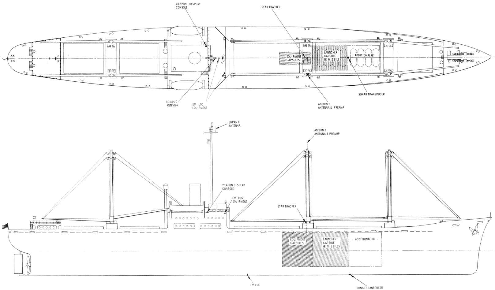
Figure II-2. Multilateral Force Warship - Plan and Outboard Profile
